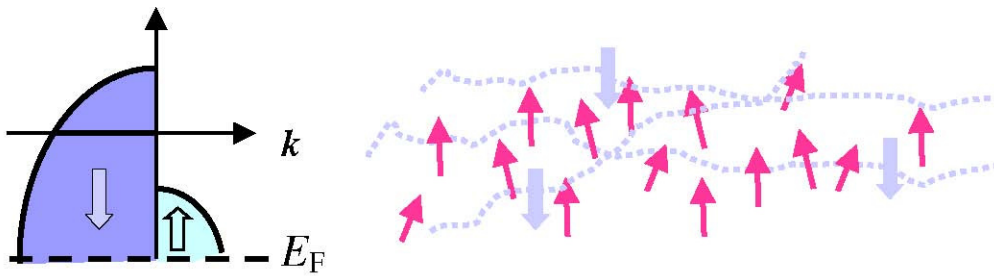
FIG.2: Pictorial presentation of carrier-mediated ferromagnetism in p-type diluted magnetic semiconductors, a model proposed originally by Zener for metals. Owing to the p - d exchange interaction, ferromagnetic ordering of localised spins (red arrows) leads to the spin splitting of the valence band. The corresponding redistribution of the carriers between spin subbands lowers energy of the holes, which at sufficiently low temperatures overcompensates an increase of the free energy associated with a decrease of Mn entropy associated with the spin ordering.
