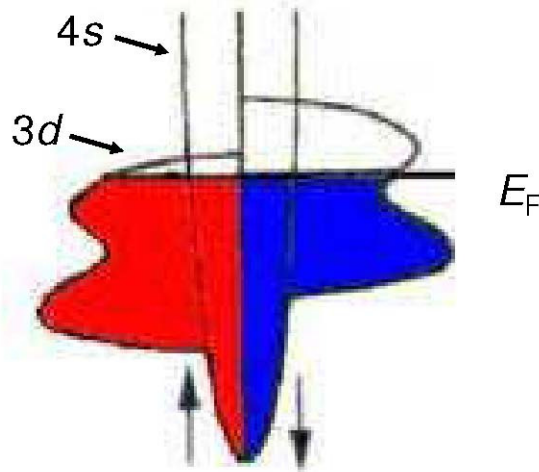
FIG. 3: Pictorial presentation of the Stoner mechanism accounting for ferromagnetism of itinerant magnetic moments. Owing to the Mott-Hubbard insulator-to-metal transition the 3d orbitals become delocalised and form bands. As long as these bands remain narrow, an increase of kinetic energy associated with redistribution of electrons to the majority spin subband does not overcompensate a lowering of the Coulomb energy occurring if electrons are spin polarised.
